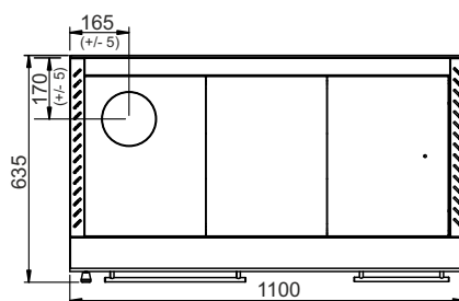
BIO-PEK B 23-L
