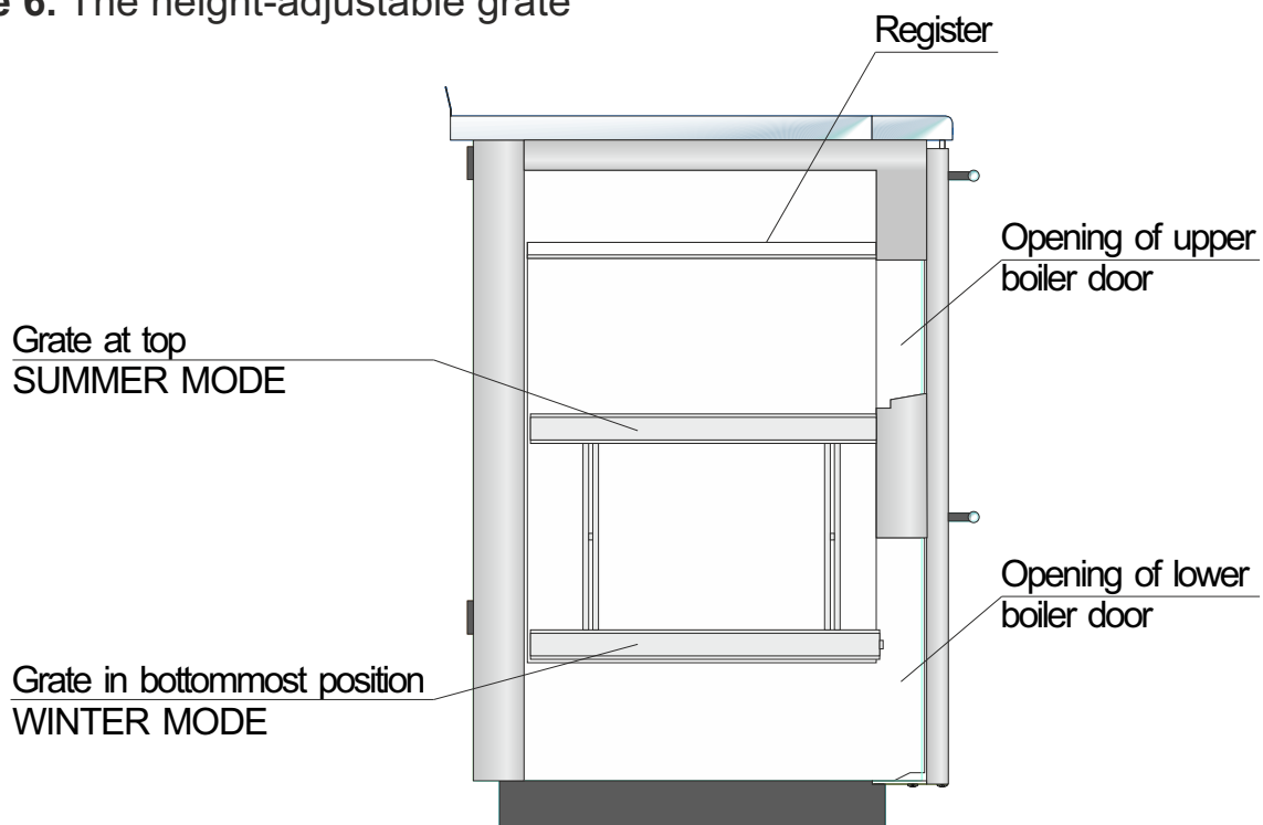
Figure 6. The height-adjustable grate
