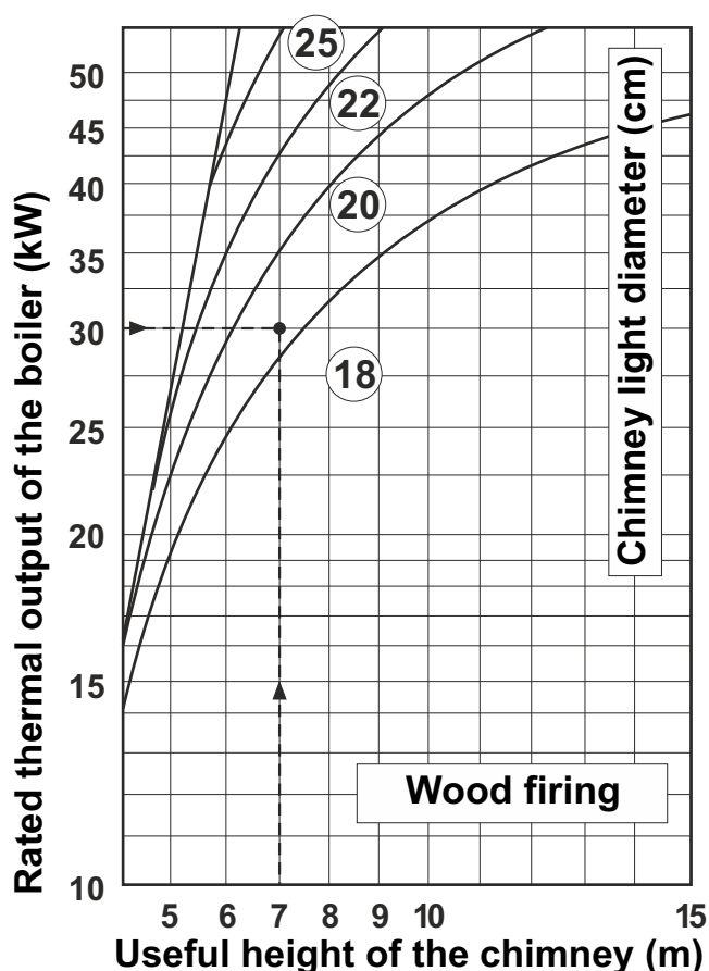
Figure 1. Dimensioning of the chimney for BIO-PEK B
