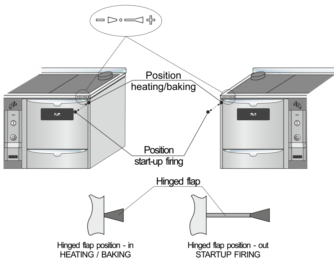
Figure 3. Handling with the hinged flap of the BIO-PEK B
