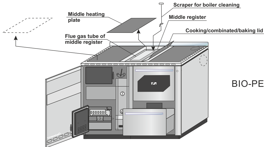
Figure 8. Exchange surfaces cleaning - BIO-PEK B-D (applies to BIO-PEK B - L)
