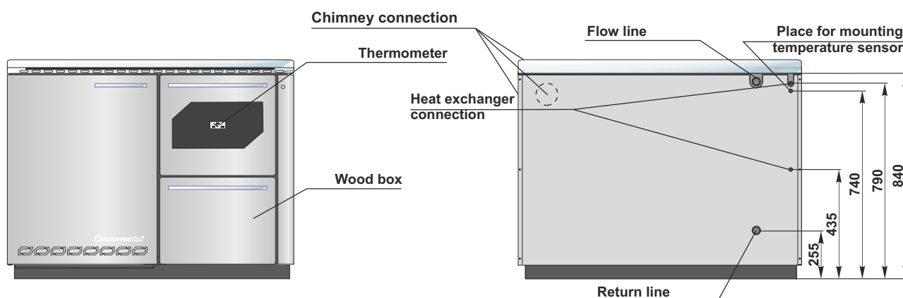
Figure 10. - BIO-PEK B - D (applies to BIO-PEK B - L)
