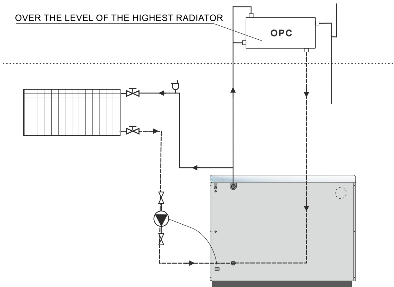
Scheme 1. Connecting an BIO-PEK B - L (applies to BIO-PEK B - D)
